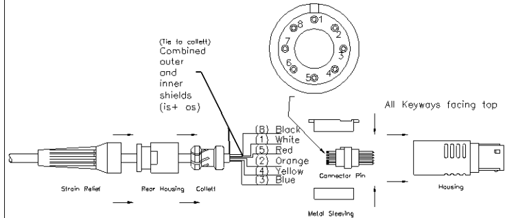
Connector Pin Rear View
