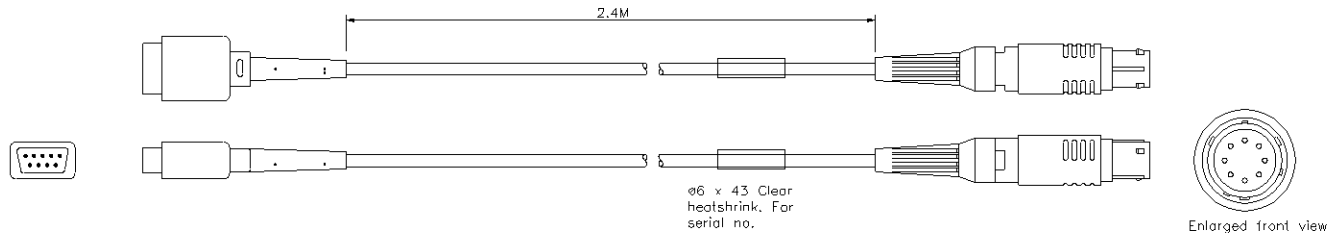
P956E8 Extension cable
