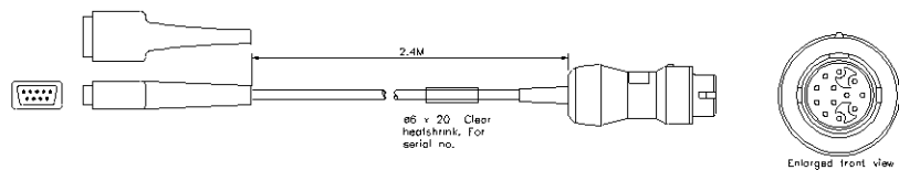
D-Type Female 9 Pin
