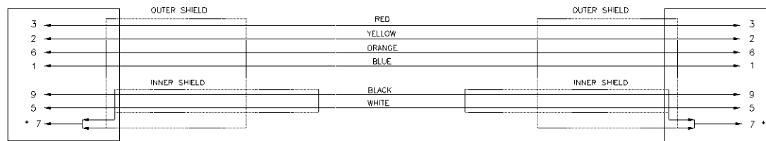
D-Type Female 9 Pin
