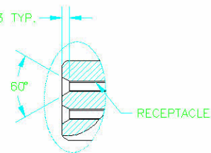
SECTION VIEW - RECEPTACLE
