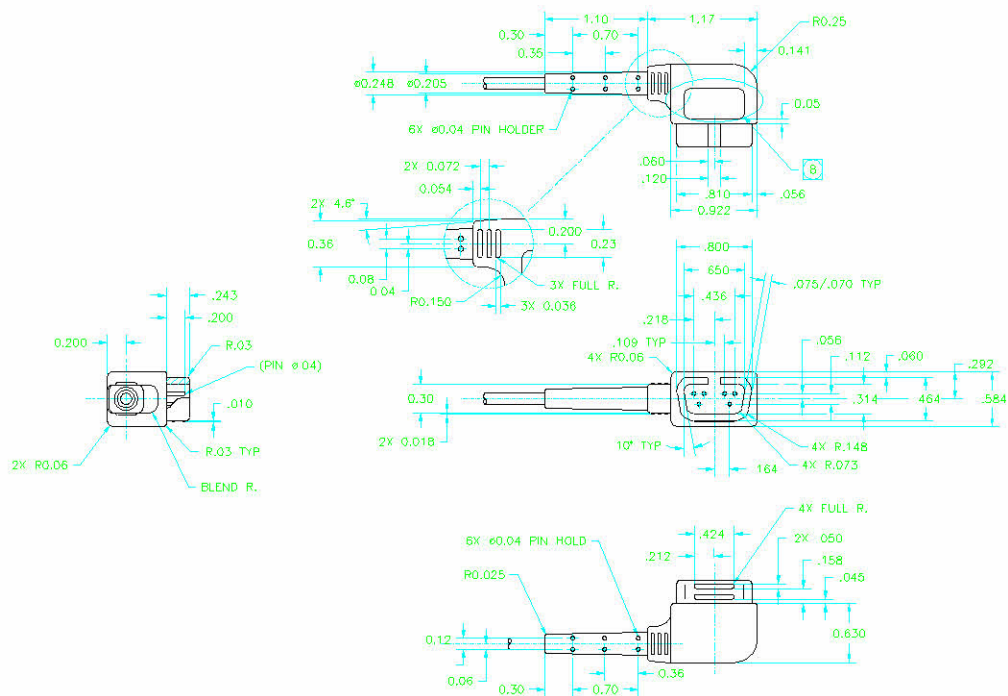
DETAIL B (DB9M)
