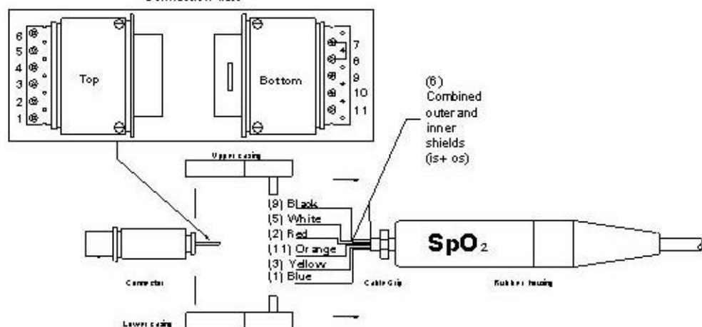
Connection view
