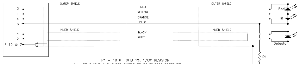
Thorkom female 12 pin
