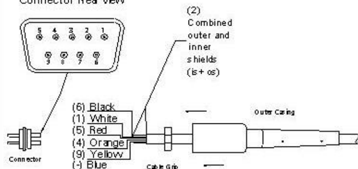
Connector Rear View
