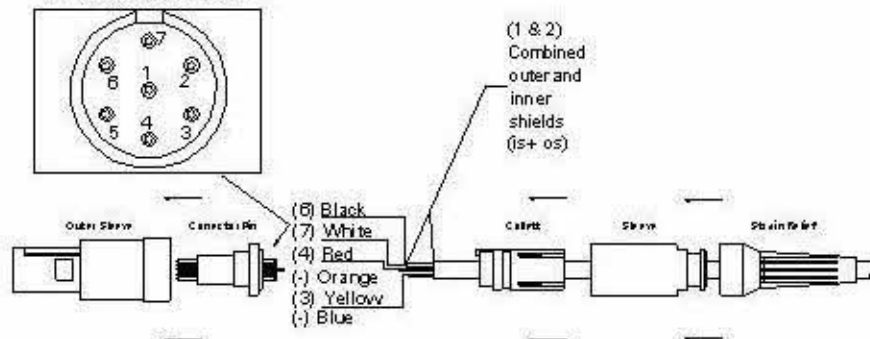
Connector Rear View
