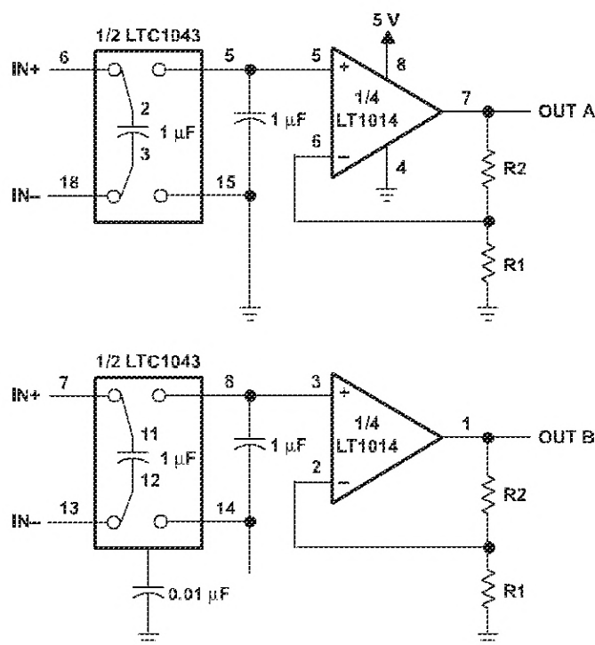
Figure 32. 5-V Single-Supply Dual Instrumentation Amplifier
