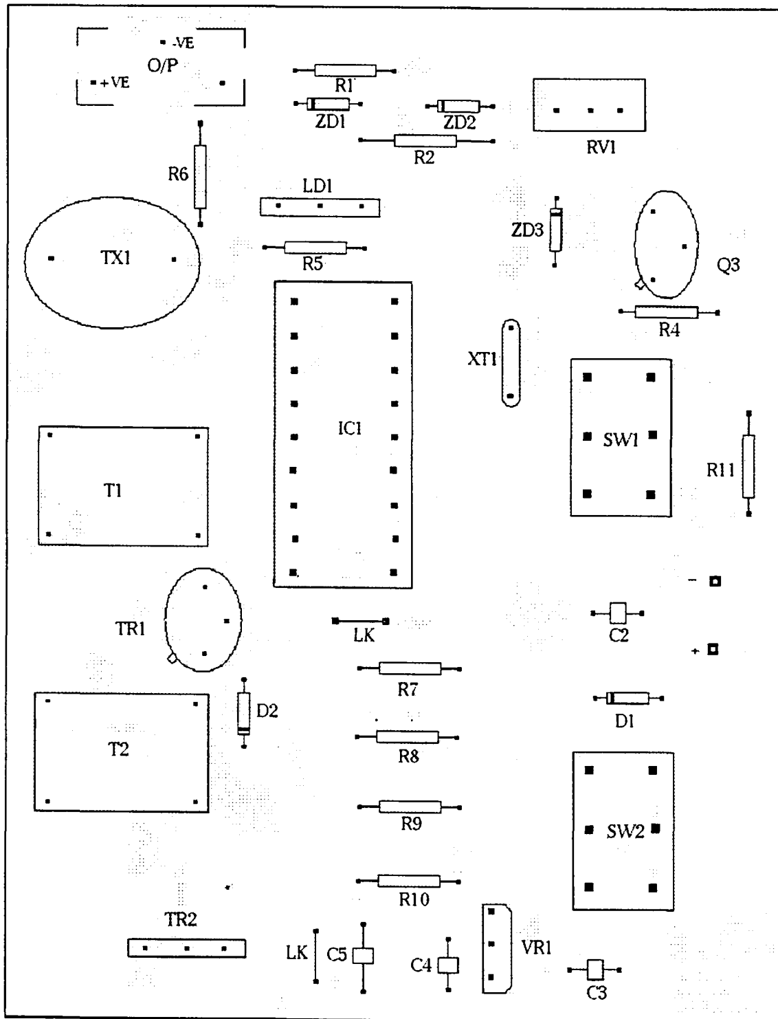
MICROSTIM DB COMPONENT LAYOUT (PKC 16F3-0)
