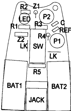
COMPONENT LOCATIONS
