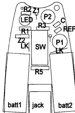
COMPONENT LOCATIONS
