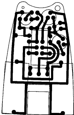
PCB TRACK LAYOUT
