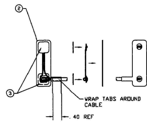
BOTTOM ENVELOPE/LIGHT BLOCKER ASSEMBLY
