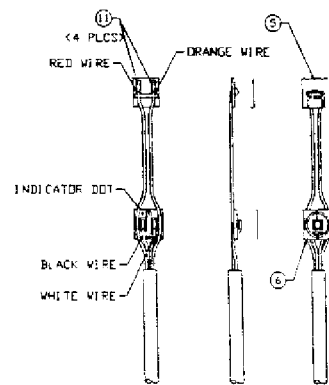
CABLE/DET/ENT ASSEMBLY
