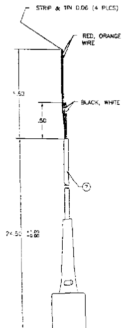
WIRE CUT LENGTH
