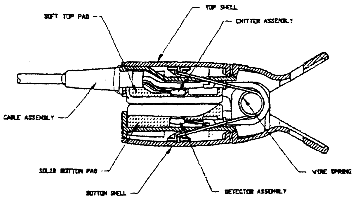
SECTION VIEW, FINGER PROBE
