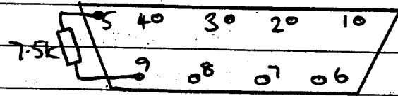
PINSIDE VIEW
