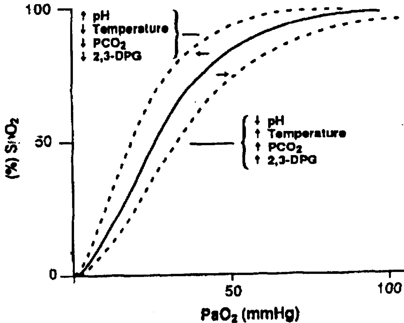
Oxyhemoglobin Dissociation Curve
