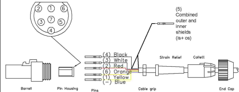
Pin Housing Rear View
