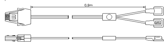
Compushield M-6
