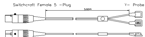
Switchcraft Female 5 pin
