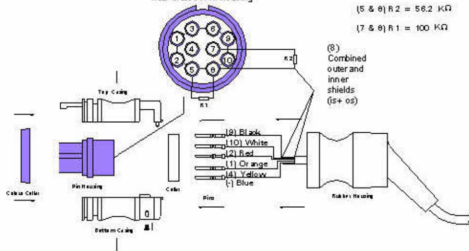
Rear View of Pin Housing
