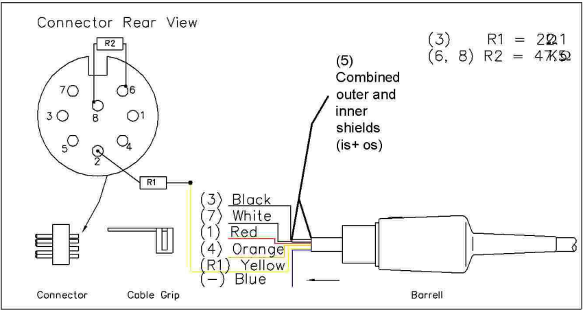
Pre-manufactured cable
