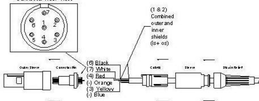
Connector Rear View
