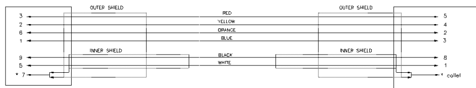
D-Type Female 9 Pin
