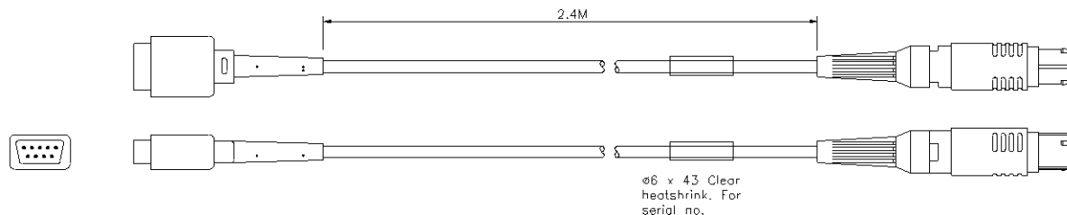
P956E8 Extension cable
