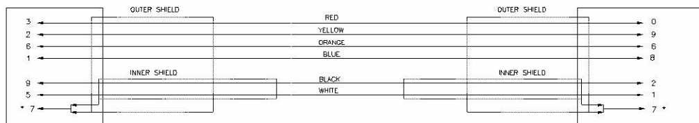
D-Type Female 9 Pin
