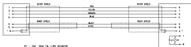
D-Type Female 9 Pin
