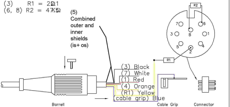
Connector Rear View
