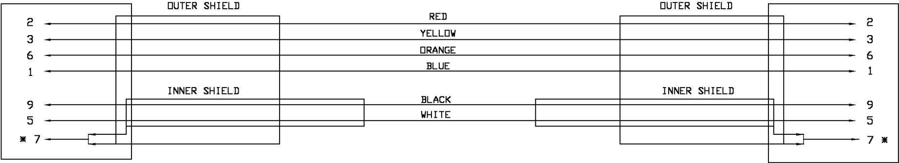
D-Type Female 9 Pin
