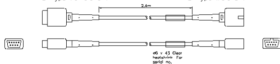
D-Type Female 9 Pin
