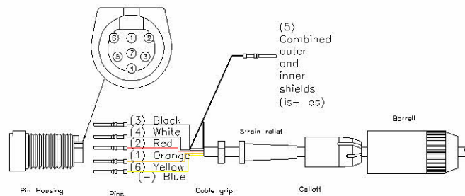
Pin Housing Rear View
