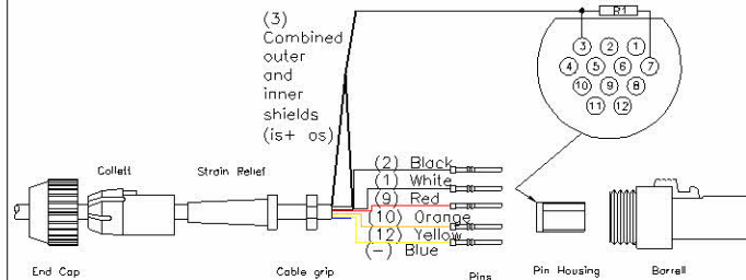
Pin Housing Rear View
