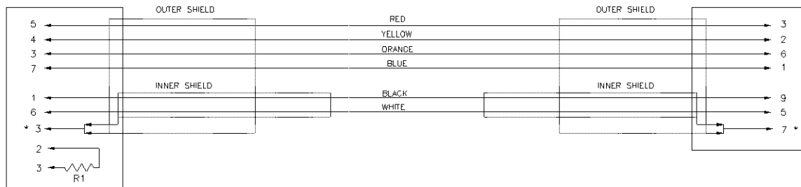
D-Type Female 9 Pin
