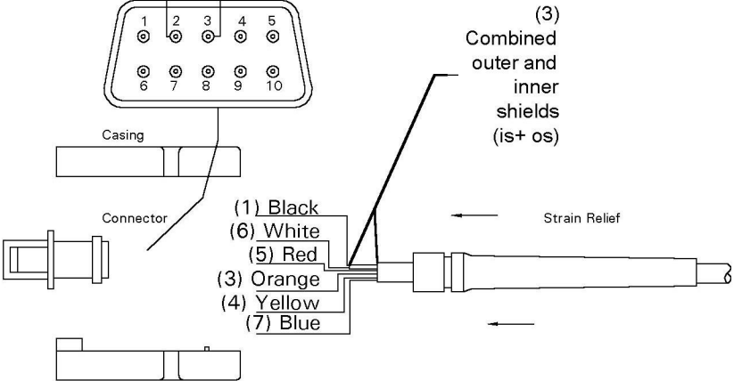
Connector Rear View
