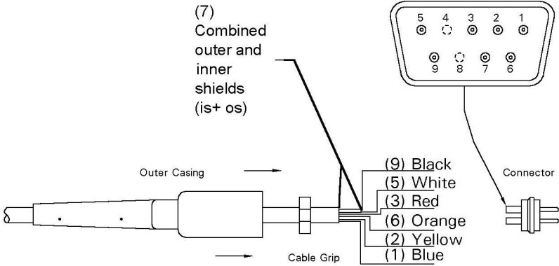
Connector Rear View
