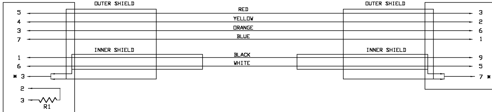
D-Type Female 9 Pin
